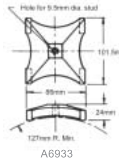
Utility clamps
